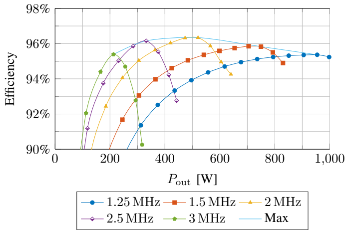
Fig. 10: Efficiency of the prototype for V_{in} = 48 V and D = 0.25 .
